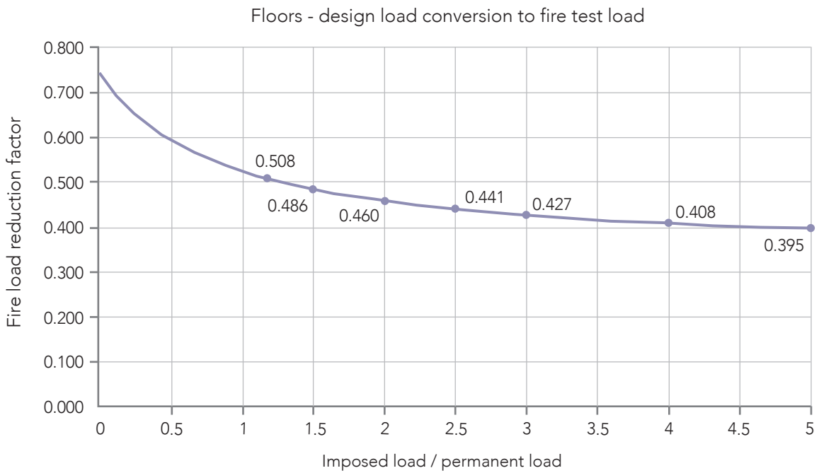
Figure 2: Variation of the fire load reduction factor \eta_{fi} for different UK floors
